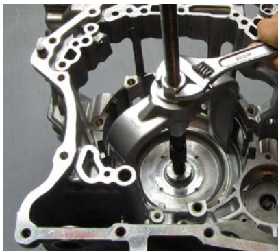
(5) Remove the bushing using a blind hole puller
