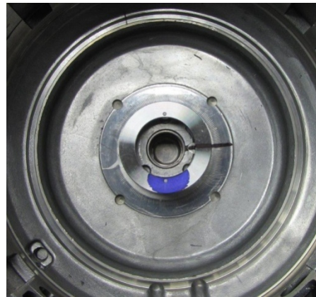
(10) Place the sleeve onto the case with marks aligned, and blue tinted hole at 6:00 o'clock
