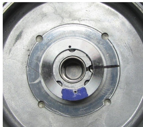
(12) Drill a .062" / 1.58mm hole .385" / 9.78mm deep, drive the roll pin in to prevent the sleeve from rotating, remove any burrs
