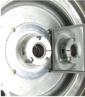
(7) Alto 129355A Sleeve Installation , Mark the case to insure proper alignment of oil circuit
